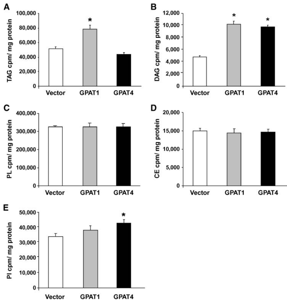
Fig. 5. GPAT4 increases [ ^{14}\text{C} ]oleate incorporation into DAG in Cos-7 cells. Cos-7 cells were transfected with pcDNA3.1, Gpat1 , or Gpat4 for 17 h and incubated with trace [ ^{14}\text{C} ]oleate for 3 h ( n = 3 ). A: Label incorporation into cellular triacylglycerol (TAG). * P < 0.05 compared with vector. B: Label incorporation into cellular DAG. * P < 0.001 compared with vector. C: Label incorporation into total phospholipid (PL). D: Label incorporation into cholesteryl ester (CE). E: Label incorporation into phosphatidylinositol (PI). * P < 0.05 compared with vector. Data are shown as means \pm SEM.
