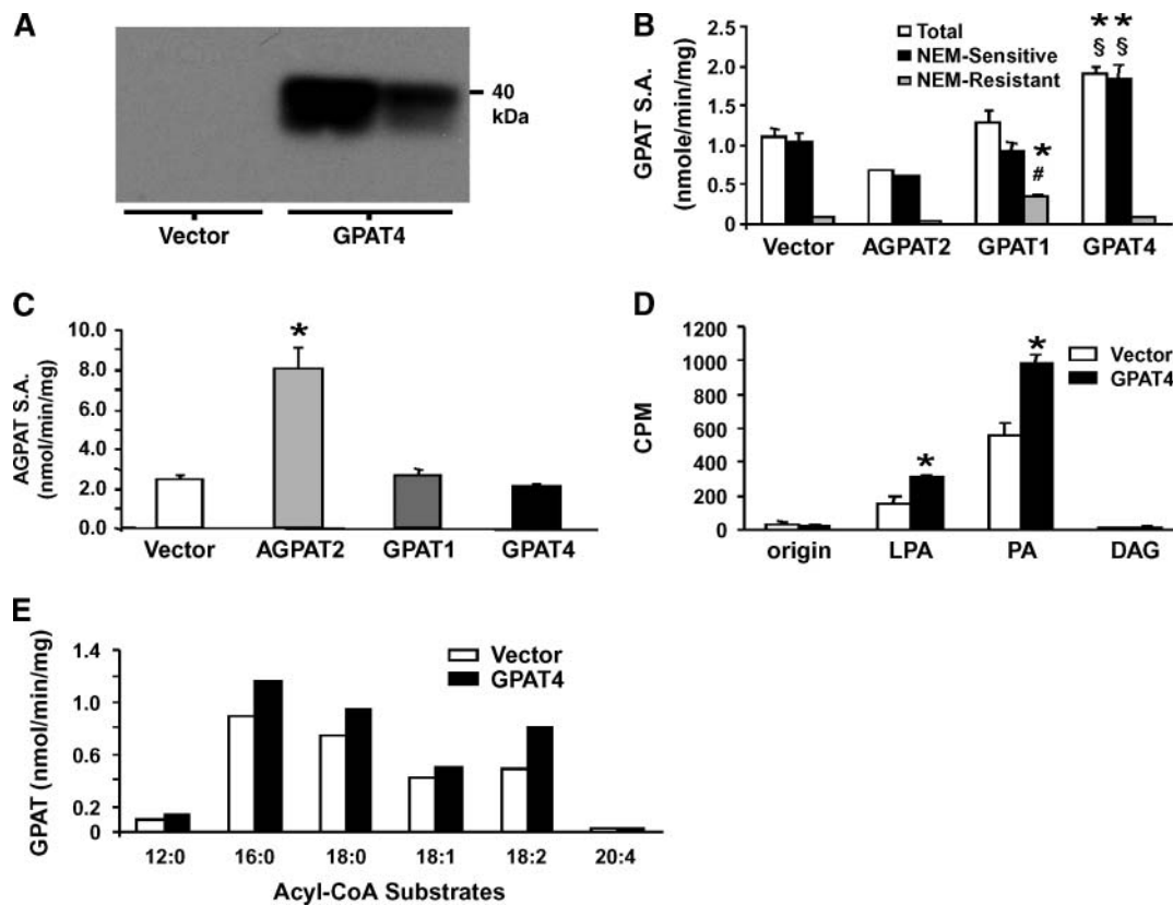
Fig. 3. Overexpression of GPAT4 in Cos-7 cells increases NEM-sensitive GPAT activity. Cos-7 cells were transfected with pcDNA3.1 vector, Atpat2 , Gpat1 , or Gpat4 . A: Immunoblot of Cos-7 cell total membrane fractions against the FLAG epitope (two independent transfections). B: GPAT specific activity (S.A.) in Cos-7 total membrane fraction (vector, n = 13; GPAT4, n = 12; GPAT1, n = 4; AGPAT2, n = 2). * P < 0.0001 compared with vector; # P < 0.0001 compared with GPAT4; § P < 0.0001 compared with GPAT1. C: AGPAT specific activity in Cos-7 cell total membrane fraction (n = 3). * P < 0.01 compared with vector. D: Radiolabeled glycerolipid products from GPAT assays of Cos-7 cell total membranes were separated by TLC and quantified as described in Methods (average of two independent assays with three separate samples per assay). DAG, diacylglycerol; LPA, lysophosphatidic acid; PA, phosphatidic acid. * P < 0.05 compared with vector. E: Total GPAT activity in Cos-7 total membrane preparations with different acyl-CoA substrates (60 \mu M) (average of two independent experiments). Data are shown as means \pm SEM.
