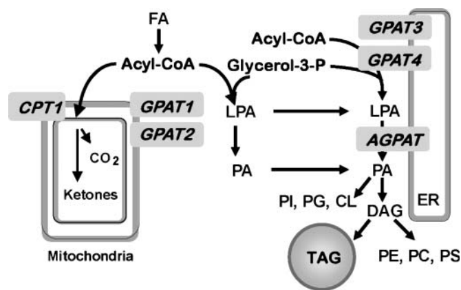
Fig. 6. Relationship of GPAT4 to other enzymes in the pathway of de novo glycerolipid synthesis. GPAT isoforms located in mitochondria (GPAT1 and GPAT2) and endoplasmic reticulum (GPAT3 and GPAT4) catalyze the initial step in the synthesis of glycerophospholipids and TAG. AGPAT isoforms catalyze the second step in this pathway by acylating LPA to form PA. Acyl-CoA used for \beta -oxidation or TAG synthesis is regulated reciprocally by carnitine palmitoyl transferase-1 (CPT1) and GPAT1 (26). CL, cardiolipin; ER, endoplasmic reticulum; PC, phosphatidylcholine; PE, phosphatidylethanolamine; PG, phosphatidylglycerol; PS, phosphatidylserine.
