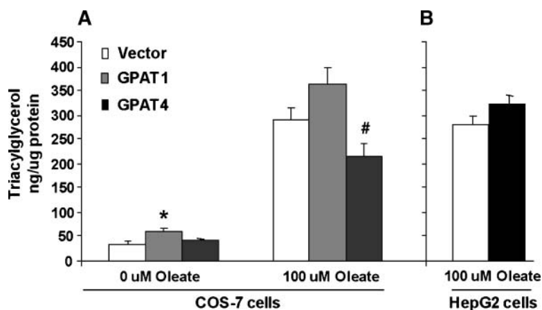
Fig. 4. Overexpression of GPAT4 in Cos-7 and HepG2 cells. A: Cos-7 cells were transfected with Gpat1 , Gpat4 , or pcDNA3.1 for 10 h before a 14 h incubation with or without 100 \mu M oleic acid. In Cos-7 cells, GPAT activities increased as shown in Fig. 3B. In HepG2 cells, NEM-sensitive GPAT activity increased by 20% ( P < 0.05 ) (0 \mu M oleate, n = 6–9; 100 \mu M oleate, n = 3). * P < 0.05 compared with vector; # P < 0.05 compared with GPAT1. B: HepG2 cells were transfected with Gpat4 or pcDNA3.1 for 12 h before a 12 h incubation with 100 \mu M oleic acid (n = 3). Data are shown as means \pm SEM.
